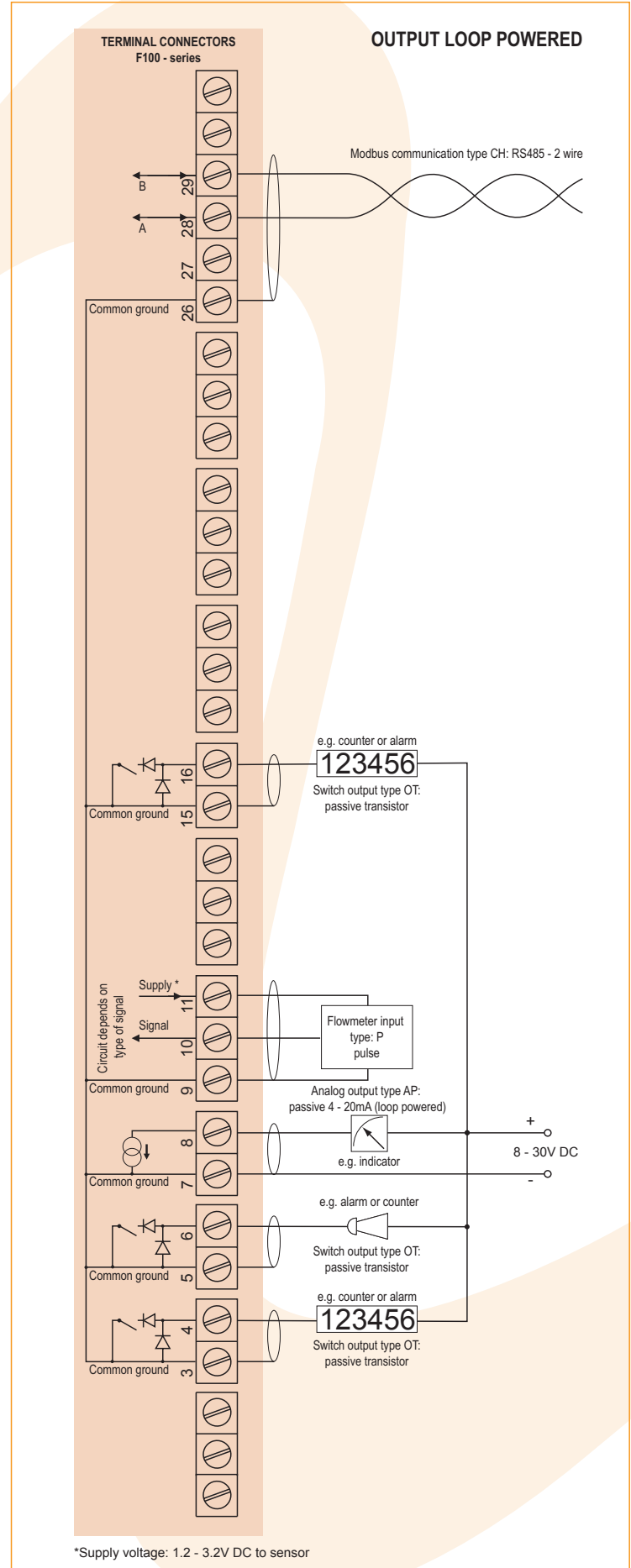
Typical wiring diagram F118-P-AP-CH-OT-PX
