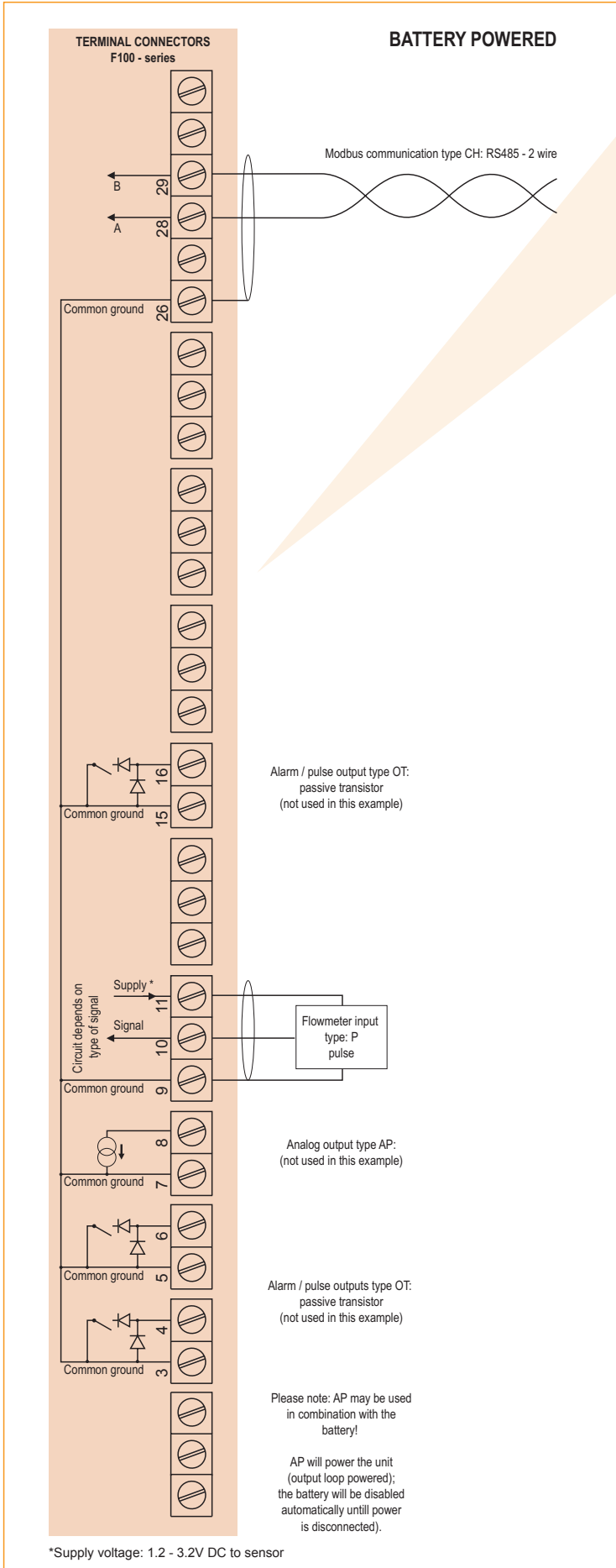
Typical wiring diagram F118-P-(AP)-CH-(OT)-PB
